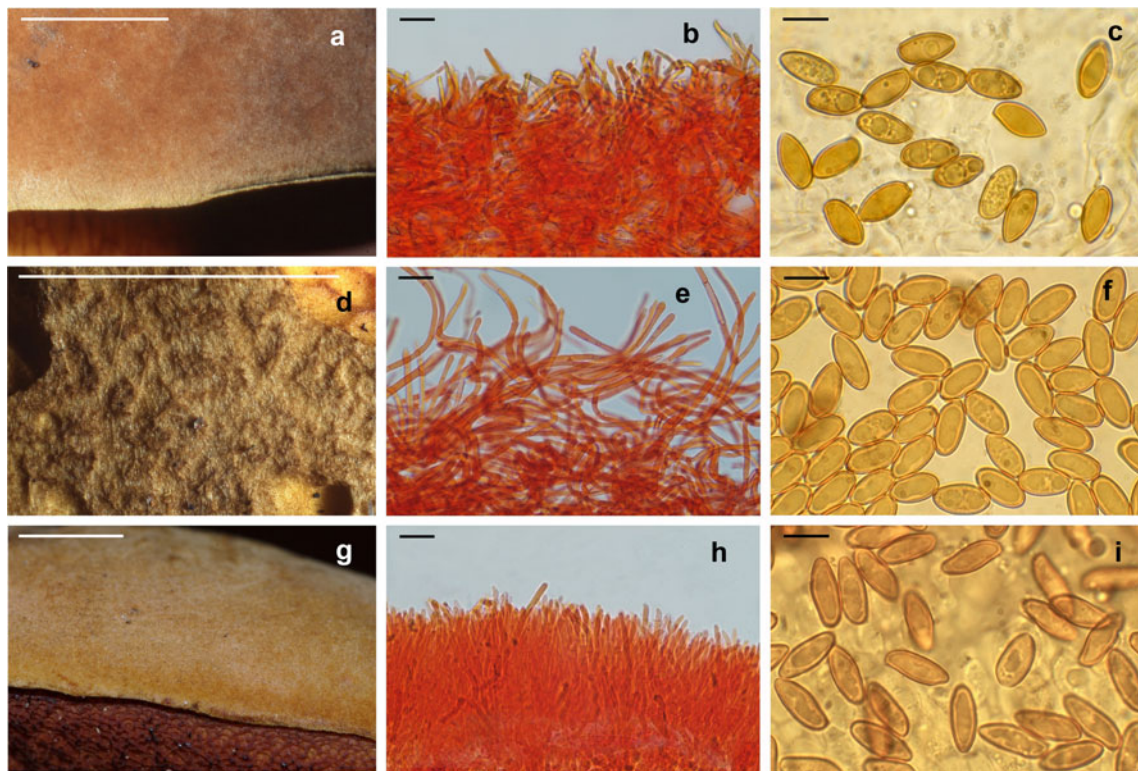
Fig. 5 Comparison among the main anatomical features of Boletus luridus (a–c, GS0875, AMB12636, MCVE17561), B. comptus (d–f, MCVE17872, GS10067, GS0978) and B. mendax (g–i, AMB12634, MCVE18095). a, d, g Magnification of the pileipellis
